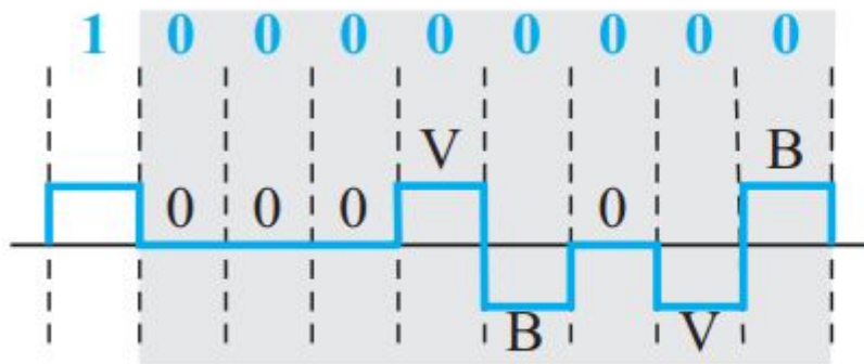
Figure 4.19 Two cases of B8ZS scrambling technique
